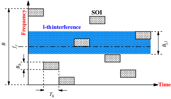
Figure 1: Distribution of desired signal and interferers over the time and frequency axes.
