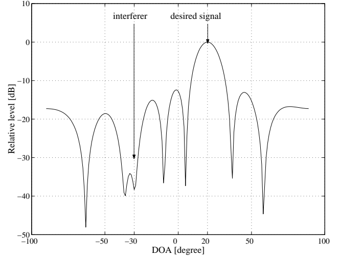
Figure 2: Antenna beampattern after 1000 iterations. (S/N=10dB, S/I=-10dB, \theta_d = 20^\circ , \theta_j = -30^\circ ).
