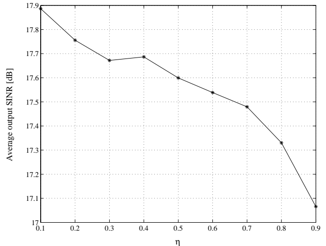
Figure 5: Average output SINR versus \eta .
