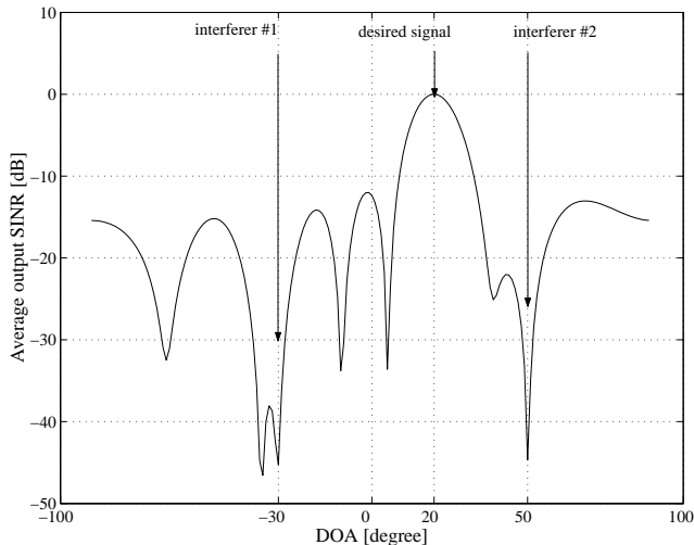
Figure 3: Antenna beampattern after 1000 iterations. ( S/N=10\text{dB} , S/I_1=S/I_2=-10\text{dB} , \theta_d = 20^\circ , \theta_{j,1} = -30^\circ , \theta_{j,2} = 50^\circ ).
