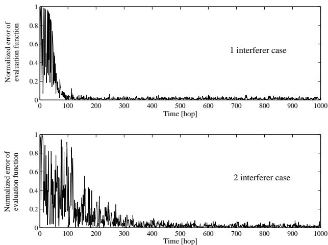
Figure 4: Convergence curves with one or two interferences.
