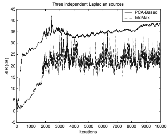
Figure 5. A sample convergence plot for PCA-based and InfoMax algorithms for the separation of three Laplacian sources
