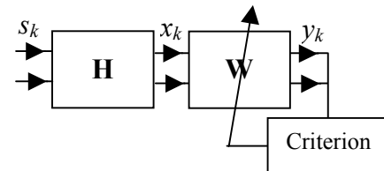
Figure 2. Schematic diagram of blind source separation
