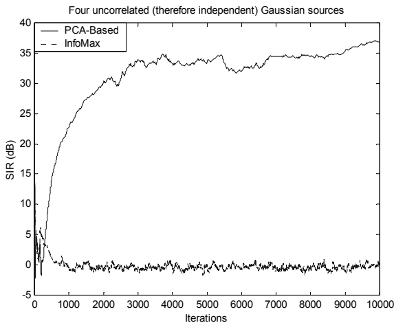
Figure 6. A sample convergence plot for PCA-based and InfoMax algorithms for the separation of four Gaussian sources
