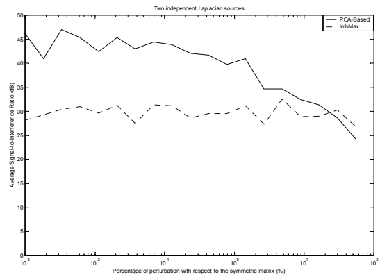
Figure 3. Average SIR(dB) vs percentage perturbation from a symmetric matrix
