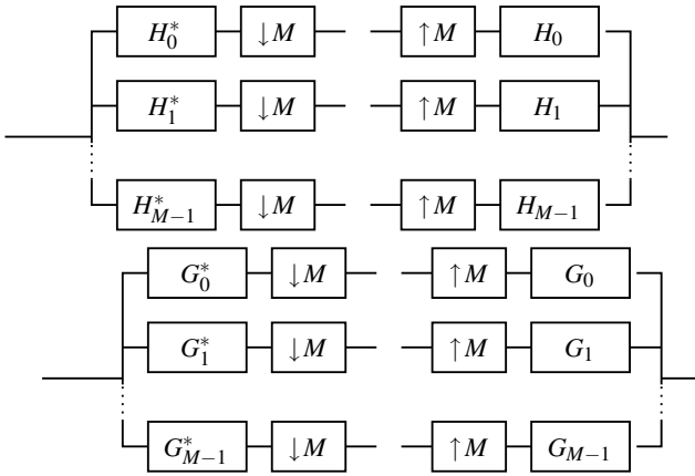
Figure 1: Analysis/synthesis M -band para-unitary filter bank
