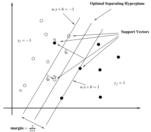
Figure 2: SVM Classifier.
