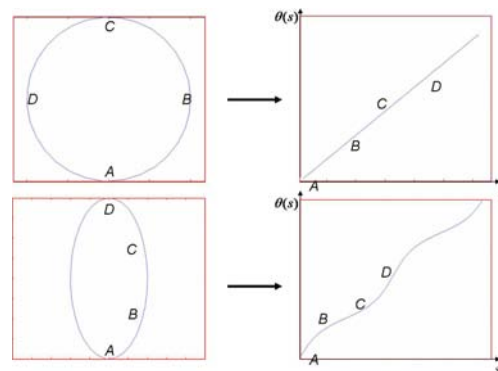
Figure 3: Examples of shapes and corresponding angle functions.
