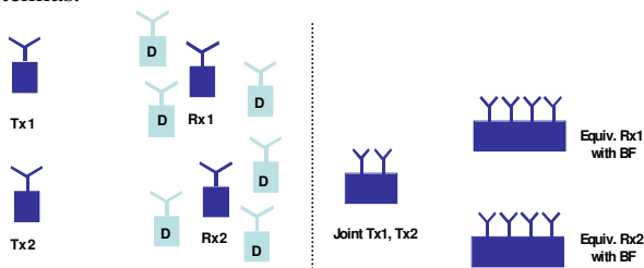
Figure 4. Left: 2x2 system with 3 dummy sensors per receive sensor. Right: Equivalent MIMO system
