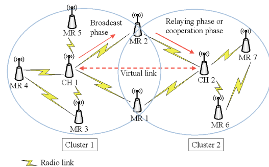
Fig. 1. Diamond topology with virtual link.
