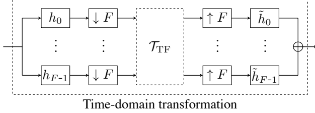
Fig. 1. Analysis/synthesis filter bank
