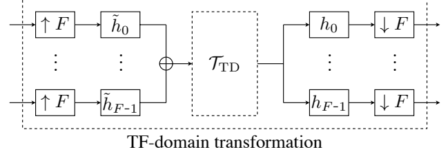
Fig. 2. Synthesis/analysis filter bank
