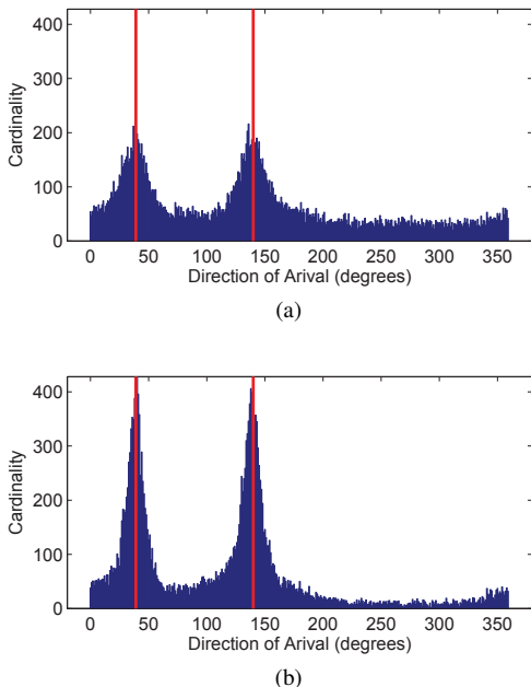
Fig. 2. Histogram of instantaneous DOA estimates obtained using MUSIC with (a) the traditional input and (b) the input derived by the proposed methodology, for a simulated recording of two active sources at 39^\circ and 140^\circ with reverberation time of T_{60} = 400 ms and 20 dB SNR. The vertical lines correspond to the true sources' DOAs.
