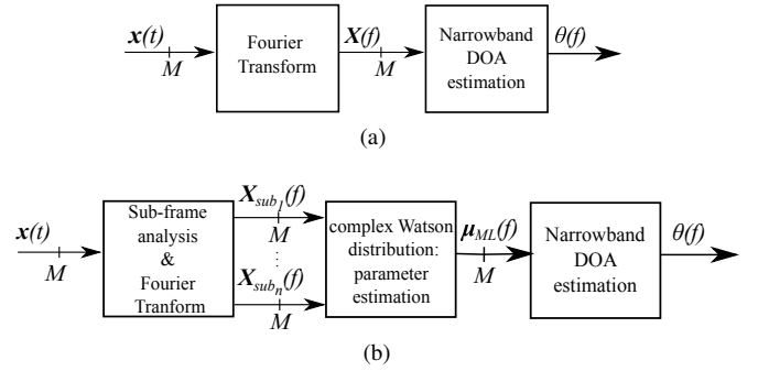
Fig. 1. Block diagram for the estimation of the instantaneous DOA for frequency point f at time frame t , using (a) the traditional input from the microphones and (b) our proposed methodology.
