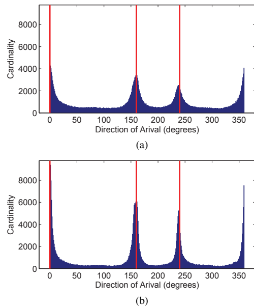
Fig. 5. Histogram of instantaneous DOA estimates obtained using MUSIC with (a) the traditional input and (b) the input derived by the proposed methodology, for a real recording of three active sources at 0^\circ , 160^\circ , and 240^\circ in a room of reverberation time of T_{60} = 400 ms. The vertical lines correspond to the true sources' DOAs.
