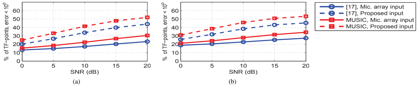
Fig. 3. Percentage of TF-points that exhibit DOA estimation error less than 10^\circ for various SNR levels for the two DOA estimation methods when using the traditional input from the array and when using the input derived by our methodology for (a) two and (b) three simultaneously active sound sources.
