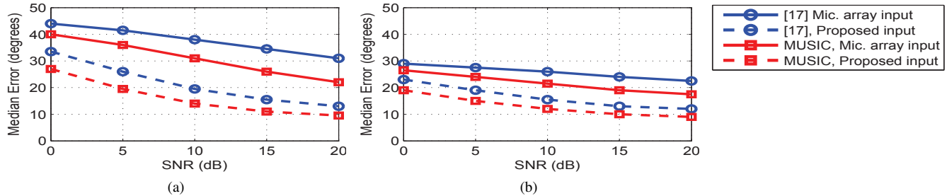
Fig. 4. Median DOA estimation error for various SNR levels for the two DOA estimation methods when using the traditional input from the array and when using the input derived by our methodology, for (a) two and (b) three simultaneously active sound sources.
