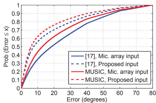
Fig. 6. Empirical Cumulative Distribution Function of the error of the instantaneous DOA estimates for the two DOA estimation methods when using the traditional input from the array and when using the one derived by our methodology, for a real recording with three active sound sources.
