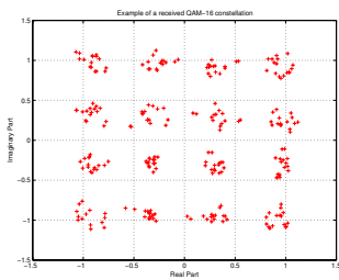
Fig. 15. Typical equalized QAM-16 constellation for CP-OFDM at 5GHz.
