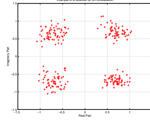
Fig. 17. Typical equalized QPSK constellation for CP-OFDM at 60GHz.
