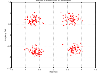
Fig. 18. Typical equalized QPSK constellation for PRP-OFDM at 60GHz.
