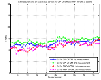
Fig. 14. Typical C/I for equalized and phase corrected constellation at 60GHz.
