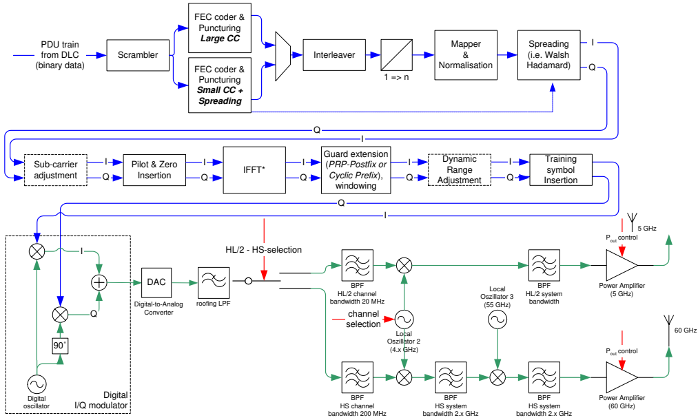
Fig. 2. The IST-BROADWAY transmitter architecture.
