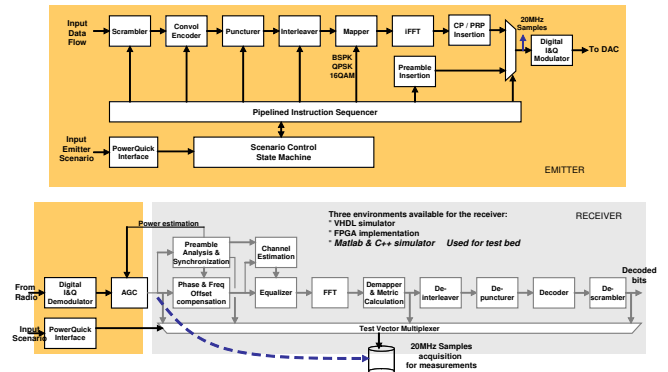
Fig. 4. Base-band implementation for the test bed.
