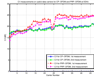
Fig. 13. Typical C/I for equalized and phase corrected constellation at 5GHz.
