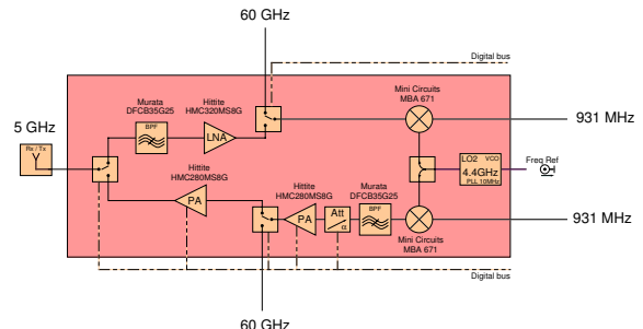
Fig. 6. RF front-end 5GHz sub-block architecture.
