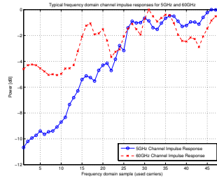
Fig. 12. Typical frequency domain channel impulse response at 5GHz and 60GHz.
