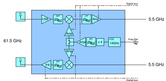
Fig. 7. RF front-end 60GHz sub-block architecture.
