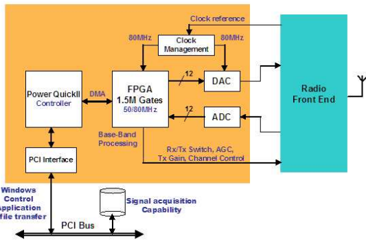
Fig. 3. Base-band Platform Overview.
