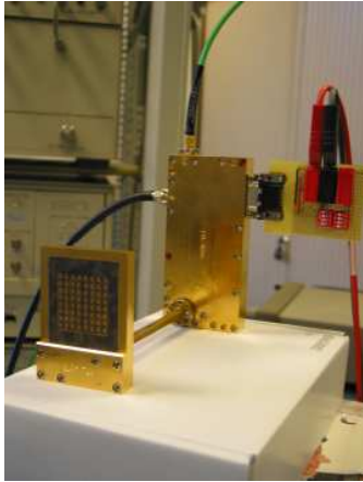
Fig. 8. 60GHz directive antenna ( > 20\text{dBi} gain) mounted on the 5-60GHz conversion block.
