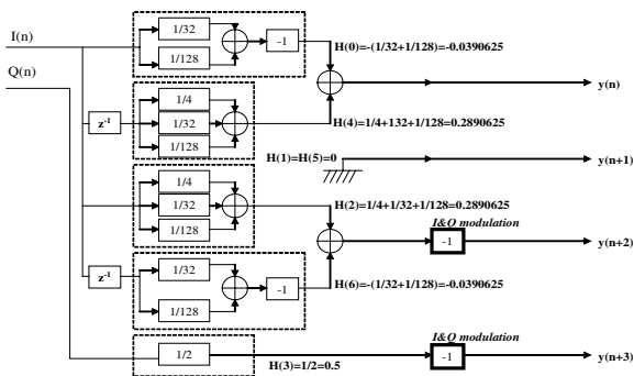
Fig. 5. Digital I/Q modulator.
