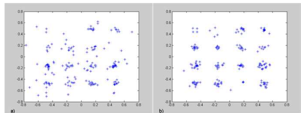
Fig. 10. Constellation diagrams for QAM-16 after C-field based channel estimation and equalisation a) without b) with band-pass filter.
