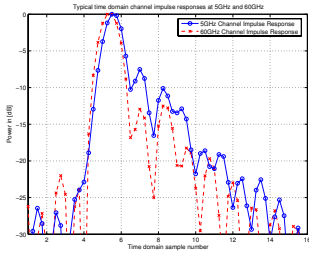
Fig. 11. Typical time domain channel impulse response at 5GHz and 60GHz.
