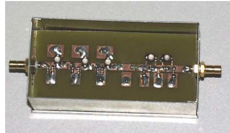
Fig. 9. Image-suppression band-pass.
