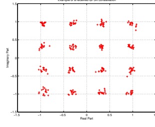
Fig. 16. Typical equalized QAM-16 constellation for PRP-OFDM at 5GHz.
