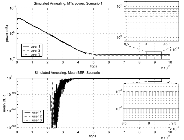
Figure 3: Performance of the Simulated Annealing in scenario 1.
