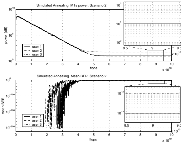
Figure 5: Performance of the Simulated Annealing in scenario 2.
