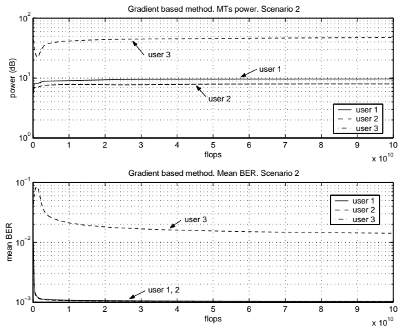
Figure 6: Performance of the gradient based algorithm in scenario 2.
