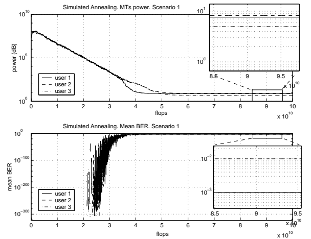
Figure 4: Performance of the Simulated Annealing in scenario 1. Power constraint in MT 1.
