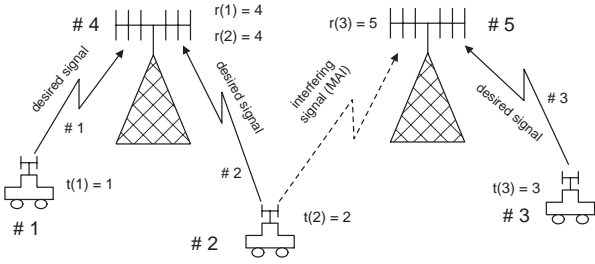
Figure 1: Typical configuration in a multiuser MIMO-OFDM scenario with 3 users or communications.
