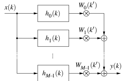
Figure 2: Low delay filter-bank with time varying gain factors.
