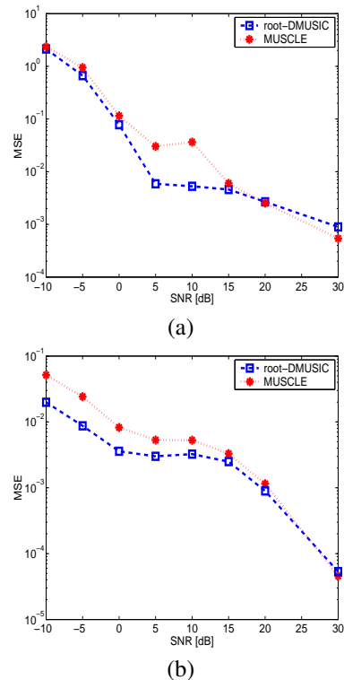
Fig. 3. MSE Vs. SNR, MSE Vs. SNR, N = 20 (a) angular-frequency \omega_{1,c} = 0.6 , \omega_{1,1} = 0.5 and \omega_{1,2} = 0.55 (b) damping-factor d_{1,c} = -0.2 , d_{1,1} = -0.01 and d_{1,2} = -0.2
