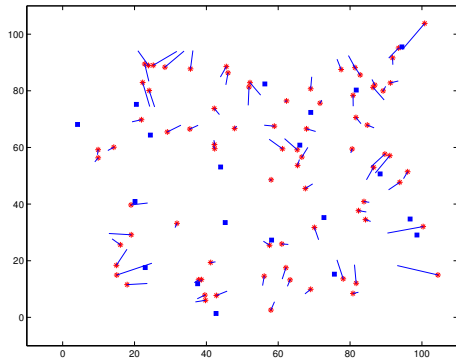
Figure 5: The 20 anchors are represented by blue squares, estimated location of the 80 nodes by a red cross, distance error in location to true position by segment.
