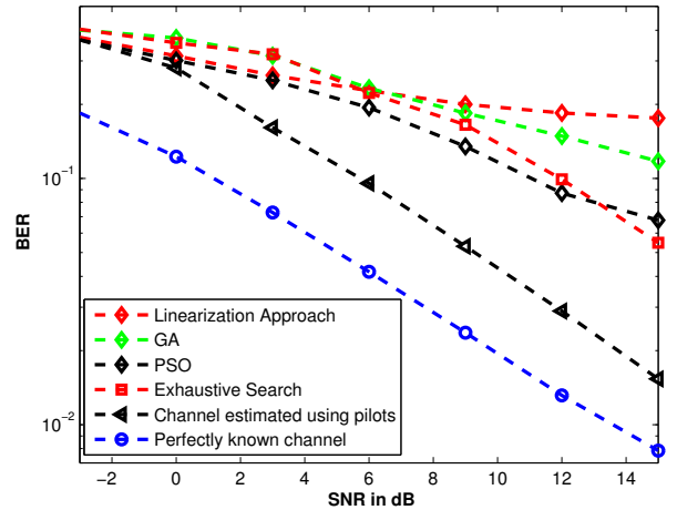
Fig. 4. Comparison of low complexity algorithms for BPSK-OFDM over a Rayleigh channel
