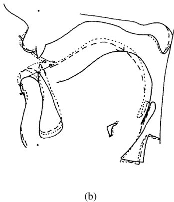
Figure 2: 2a : Mid-sagittal profiles of the vocal tract for vowel [a]. For each profile, the phonetic score, the position of the main constriction (Constric) w.r.t. the glottis and the constriction area in \text{cm}^2 are given. 2b : X-ray mid-sagittal profiles for [a]: [aba] (solid line), [maf] (dashed line), [vwa] (dotted line)
