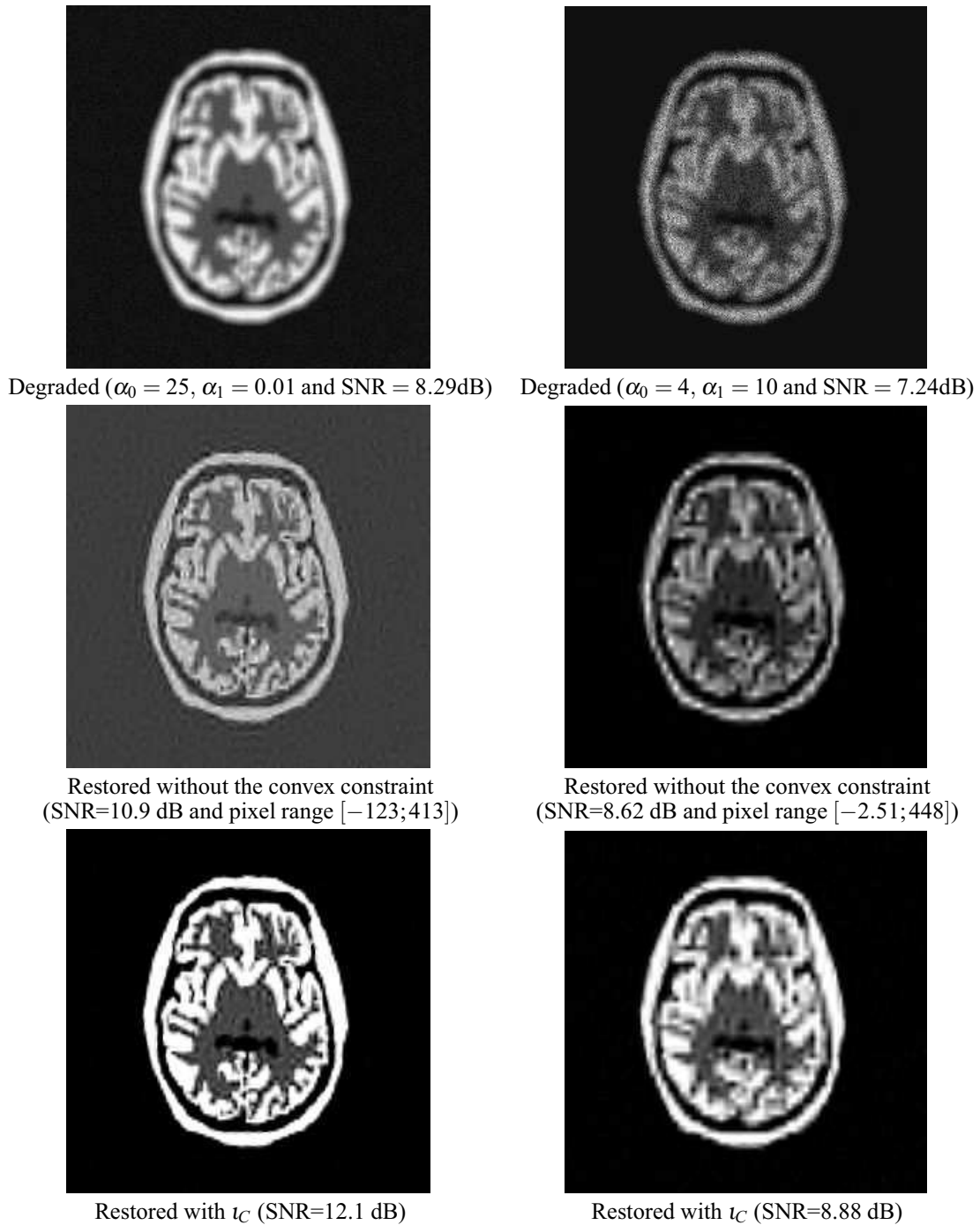
Figure 2: Restoration results on a 256 \times 256 phantom image ( M_n \equiv 10, \theta = 1/\alpha_0 ) after at most 10000 iterations.
