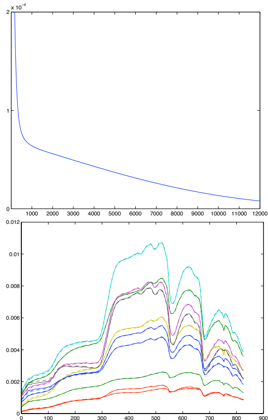
Figure 1: Frobenius \mathcal{D}(\mathbf{V}, \mathbf{W}\mathbf{H}) as a function of the number of iterations. Columns of \mathbf{V} at the end of the iterations, solid line for true values, dashed line for estimated values.
