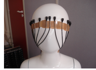
Figure 4: The 16 sensors microphone array
