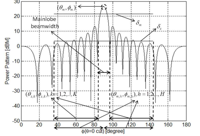
Fig. 1. Design constraints in (2). \delta_m and \delta_s define the minimum allowed mainlobe power and maximum allowed sidelobe power, respectively. (\theta_m, \phi_m) is the steering direction. (\theta_{s,k}, \phi_{s,k}), k = 1, 2, \dots, K define the sidelobe constraints. (\theta_{m,h}, \phi_{m,h}), h = 1, 2, \dots, H define the ‘highest peak at the steering direction’ constraint (last constraint in (2)).
