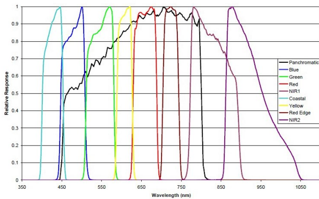
Figure 1. WV2 relative spectral radiance response (nm).
