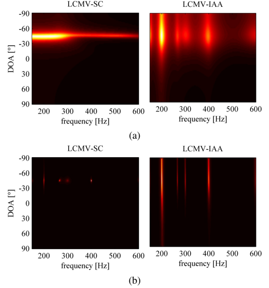
Fig. 1. Plots of the cost-functions for the LCMV-IAA and LCMV-SC methods when applied on a synthetic, multichannel, periodic signal for (a) N = 20 and (b) N = 80 .
