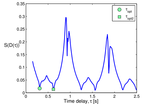
Fig. 2. Optimisation of \tau to minimise the symmetry measure, S(D(\tau)) . When evaluated on a periodic signal, \tau_{opt} and \tau_{opt2} correspond to T/3 and 2T/3 respectively.
