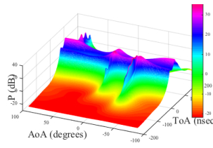
Fig. 6: 2D-MUSIC spectrum using \mathbf{R}_{\tilde{x}\tilde{x}} .
