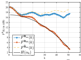
Fig. 1: Behaviour of F^{\mathbf{R}_{xx}}(k) , F^{\mathbf{R}_{\tilde{x}\tilde{x}}}(k) , F^{\tilde{\mathbf{R}}_{xx}}(k) , and H(\alpha_k) over k .
