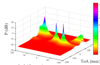
Fig. 7: 2D-MUSIC spectrum using \tilde{\mathbf{R}}_{xx} .
