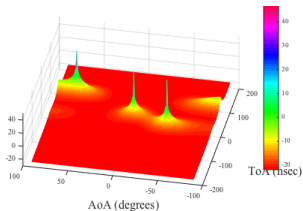
Fig. 5: 2D-MUSIC spectrum using \mathbf{R}_{xx} .
