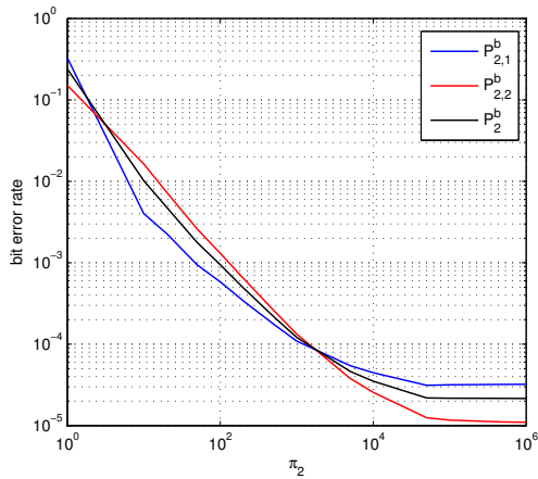
Fig. 1. Bit error rate of SU2 versus \pi_2 at NE.
