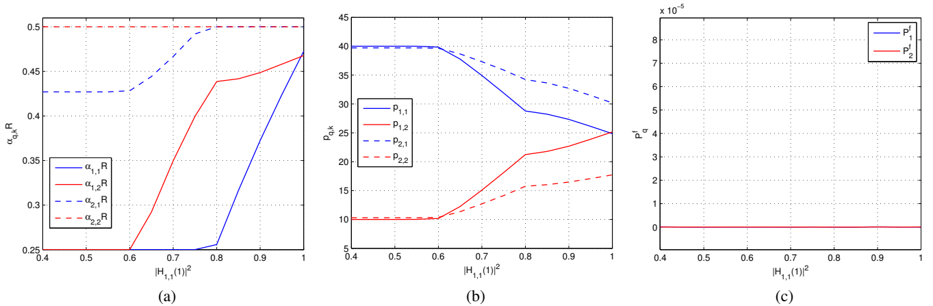
Fig. 2. (a) \alpha_{q,k} R , (b) p_{q,k} and (c) P_q^f versus |H_{1,1}(1)|^2 at NE.
