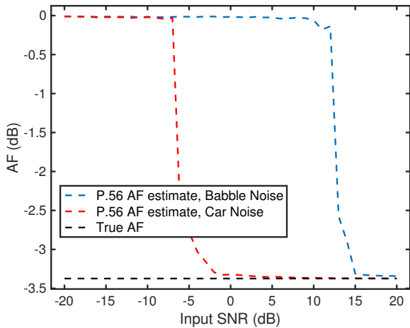
Fig. 2. The activity factor (AF) estimate of the P.56 algorithm is tested with SNR levels from -20 dB to 20 dB. One sentence from the TIMIT database [5] is used with babble noise and with car noise.
