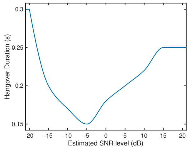
Fig. 5. The hangover duration for each SNR level is illustrated. The MSE objective function is the sum of the frame classification MSEs.
