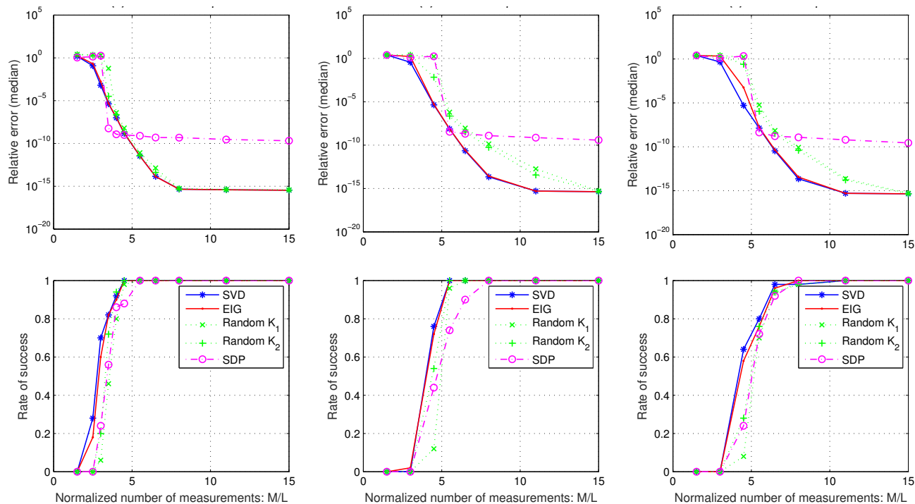
Fig. 1. Recovery performance of the joint identification of \mathbf{x} and \mathbf{h} using 5 different algorithms. The top row reports the median error, and the bottom one the percentage of tests able to recover the exact solution (up to a relative error of less than 10^{-3} ). Each column represents a different test case.
