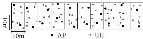
Fig. 5: Simulated multi-cell scenario
