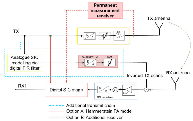
Fig. 2: Auxiliary transmitter concept for receiver protection with two options for RF impairments modeling
