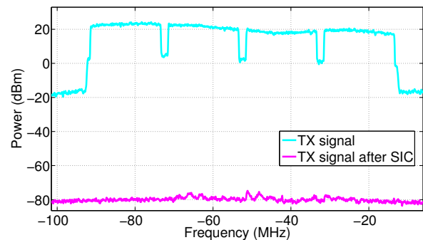
Fig. 4: SIC for a 20 dBm 4 \times 20 MHz LTE signal
