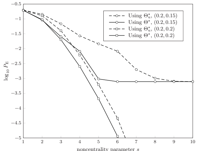
Fig. 4. Error probability performance of a network of N = 4 unlimited-capacity battery energy harvesting sensors while using unconstrained \Theta_{\text{un}}^* and adapted \Theta^* thresholds and for different (\pi_1, p_e) .
