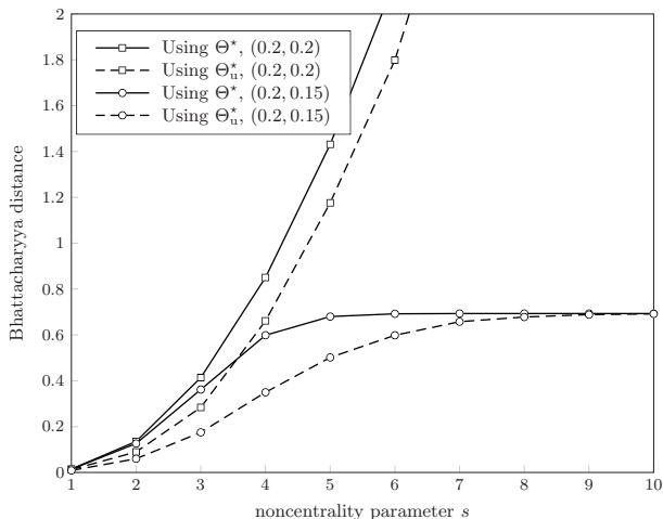
Fig. 3. Evolution of Bhattacharyya distance of an unlimited-capacity battery energy harvesting sensor while using unconstrained \Theta_{\text{un}}^* and adapted \Theta^* thresholds and for different (\pi_1, p_e) .
