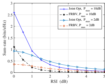
Fig. 3. Sum-rate versus residual self-interference.
