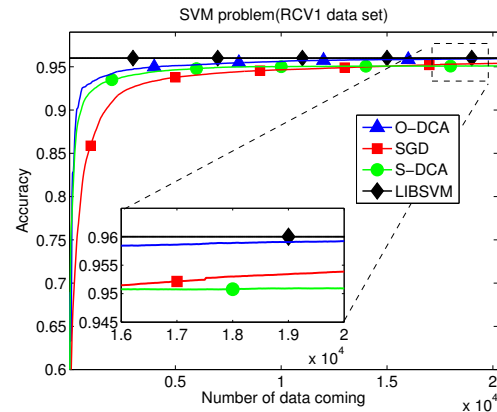
Fig. 2. Comparison of the performance of O-DCA, S-DCA, SGD, and LIBSVM on the RCV dataset in terms of iterations.
