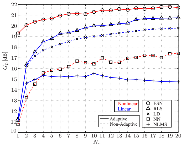
Fig. 2. Prediction gain G_p (in dB) results for a different number N_p of past speech samples (for LD: prediction order). Linear approaches (i.e., RLS, NLMS and LD) and nonlinear approaches (i.e., ESN and NN) are blue and red , respectively. The adaptive approaches (i.e., ESN, RLS and NLMS) and non-adaptive approaches (i.e., NN and LD) are shown as solid and dashed lines, respectively.
