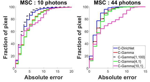
Fig. 3. CDFs of the depth absolute error, with high background ( SBR = 0.426 ). The left (resp. right) subplot corresponds to MSC equals to 10 (resp. 44) photons.
