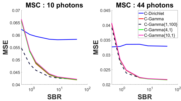
Fig. 2. MSE of \hat{R} obtained with the different competing methods as function of the SBR. The left (resp. right) subplot corresponds to MSC equals to 10 (resp. 44) photons.
