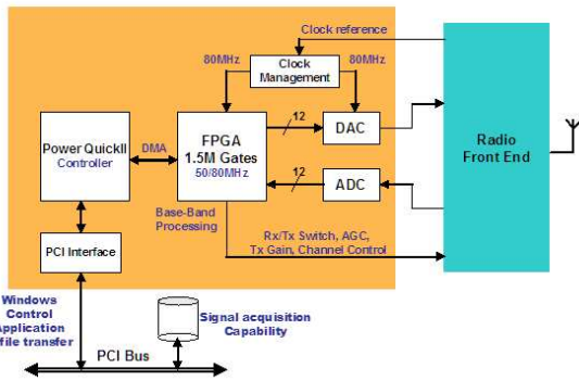
Fig. 3. Base-band Platform Overview.
