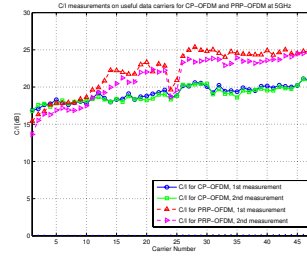
Fig. 13. Typical C/I for equalized and phase corrected constellation at 5GHz.
